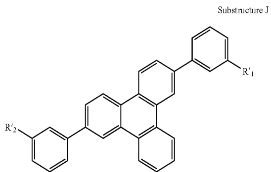
Substructure K
