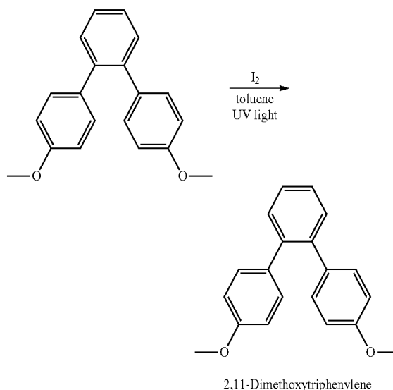
2,11-Dimethoxytriphenylene
