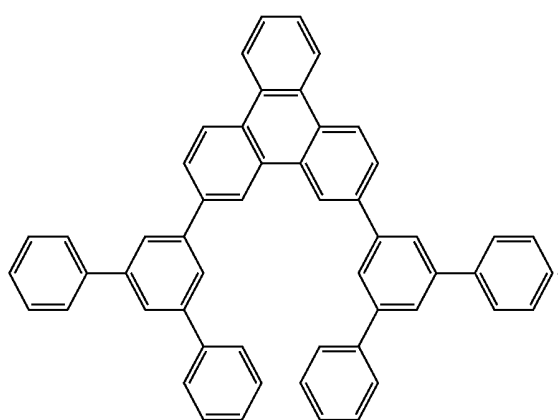
Compound 7
