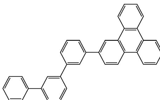
Compound 2
