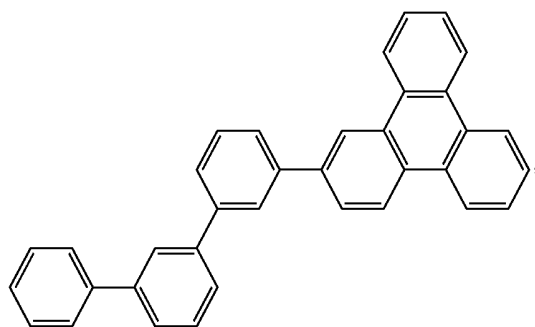
Compound 2
