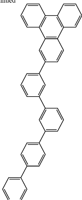
Compound 11
