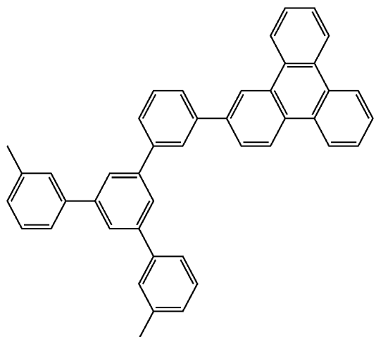
Compound 10
