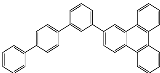
Compound 6
