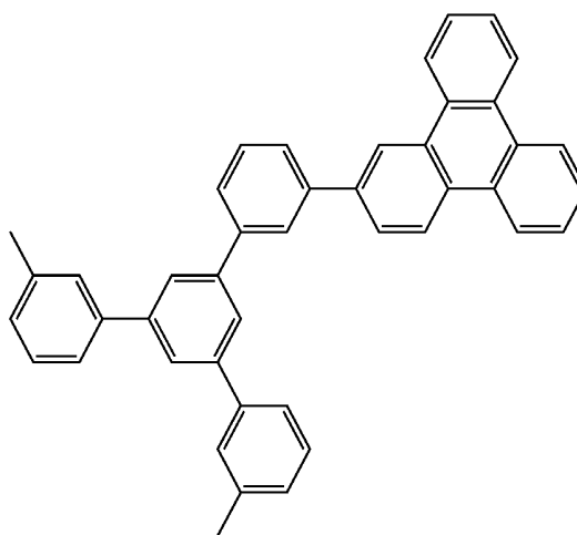
Compound 11
