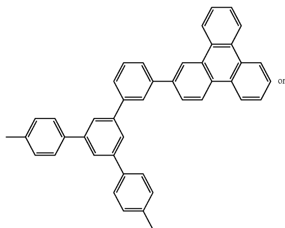
Compound 9
