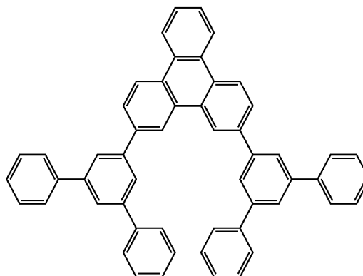
Compound 7
