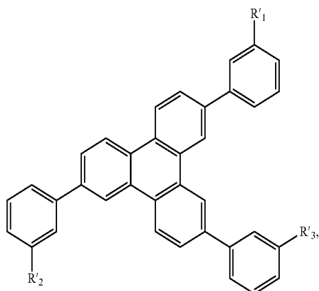
Substructure L
