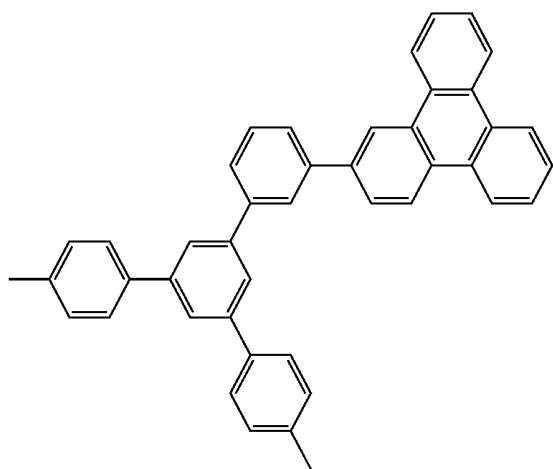
-continued Compound 9
