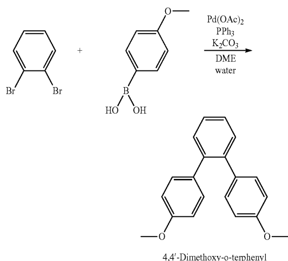
4,4'-Dimethoxy-o-terphenyl
