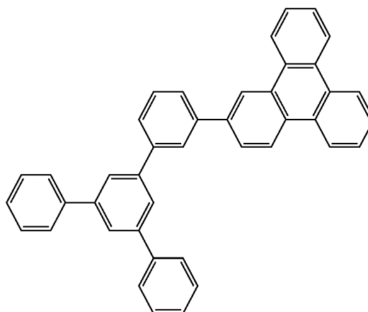
Compound 4
