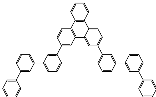
Compound 8
