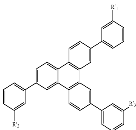
Substructure L
