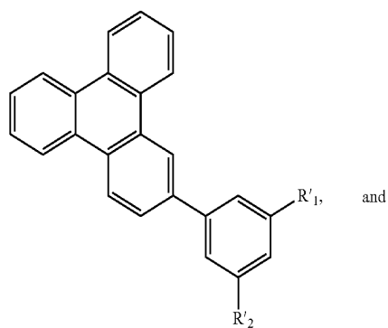
Substructure I
