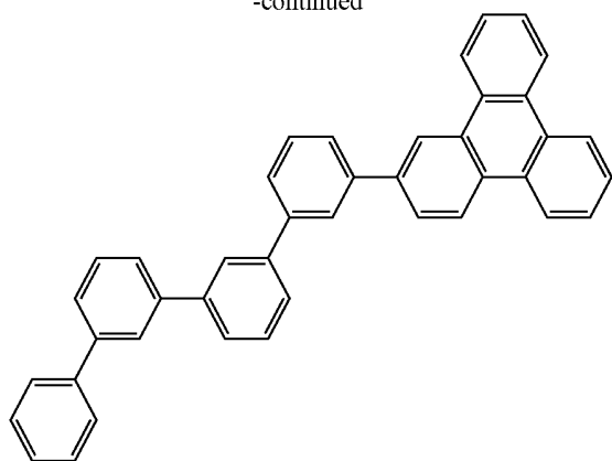
Compound 3
