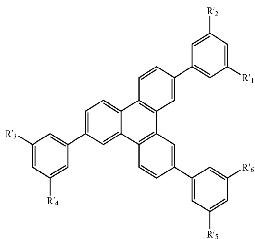
Substructure M
